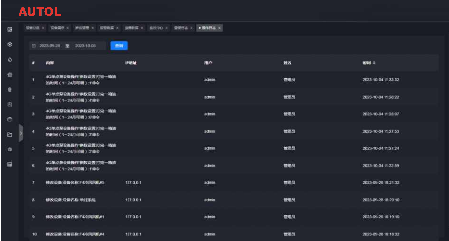
Operation log
